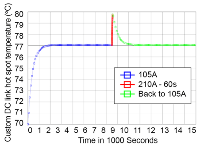
Fig. 7. Transient thermal response
